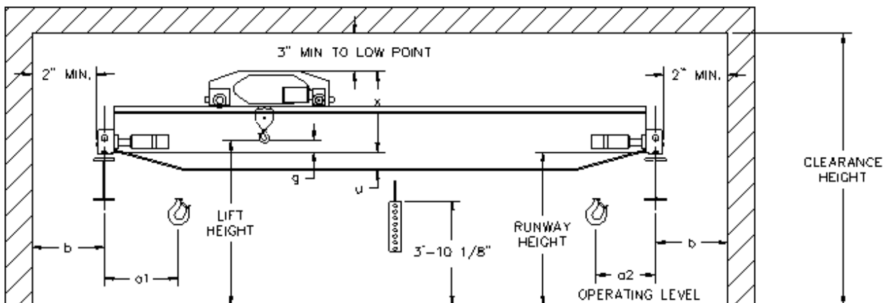
TOP RUNNING DOUBLE GIRDER CRANE
